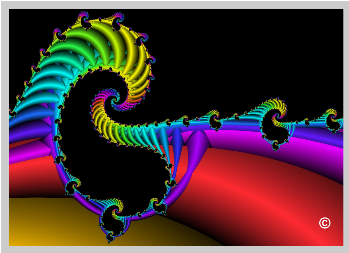
Fractal Tsunami
